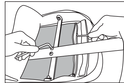
6. Remove the hex-headed screws, one key inside the back pack.
